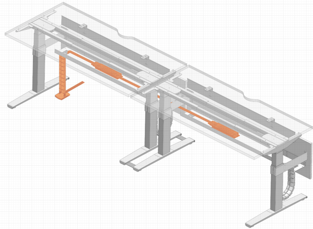
TYPICAL "I"-LEG DESK WIRING LAYOUT.
