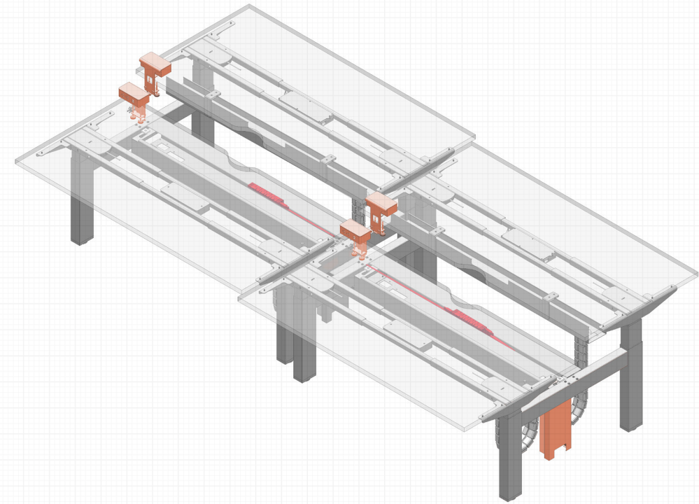
TYPICAL "H"-LEG DESK WIRING LAYOUT.
